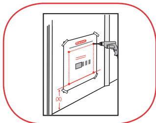
Position the template base at belly height marked on door (X). Drill holes at corners as indicated.
